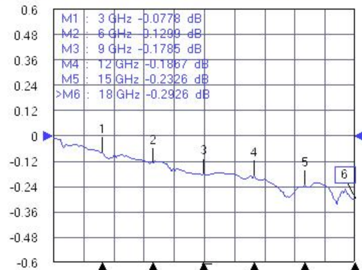
Tr3 S21 Trans LoqM RefLvl: 0 dB Res: 0.12 dB/Div
